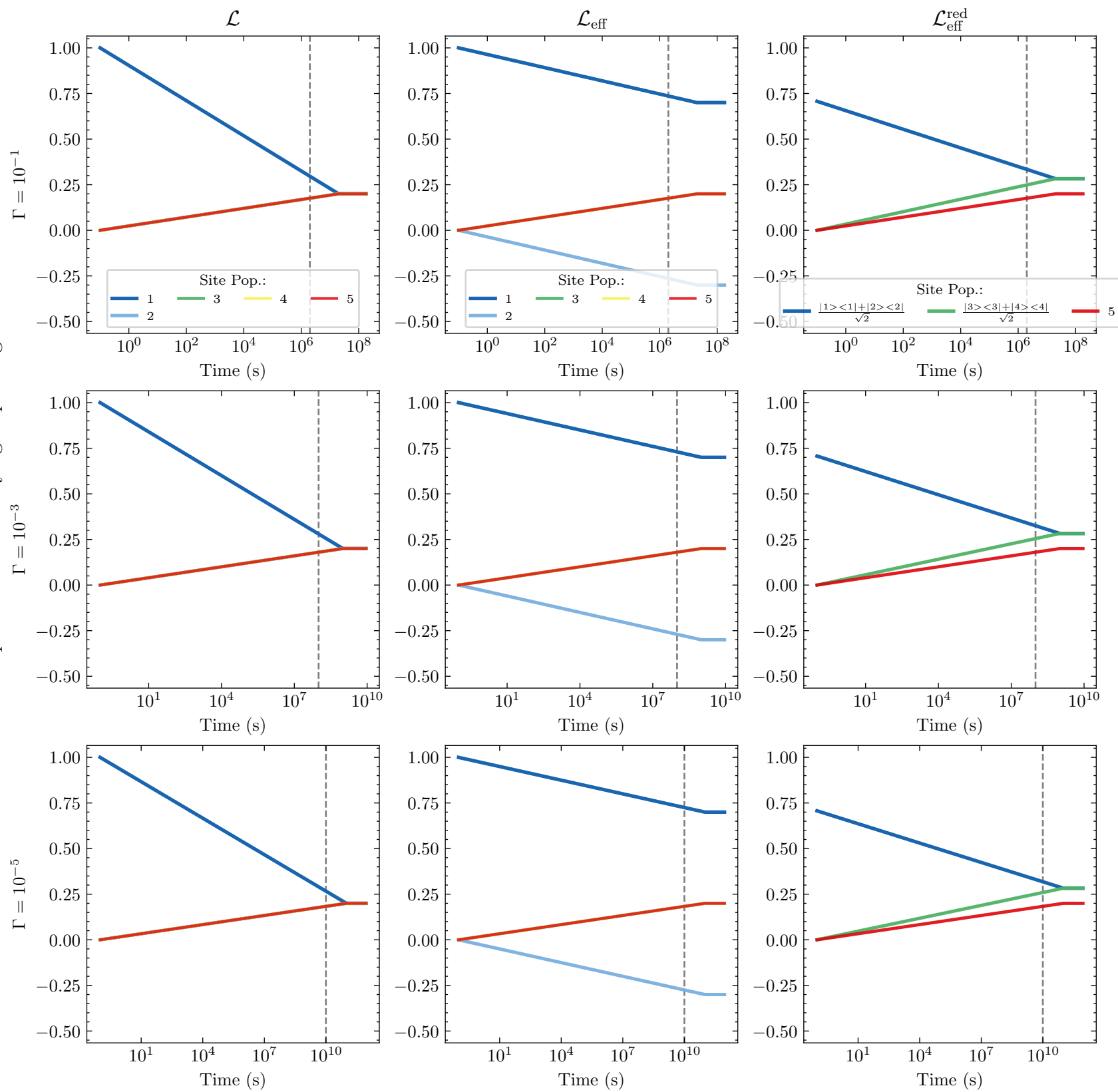
Time Evolution of Site Populations under \mathcal{L} , \mathcal{L}_{\text{eff}} , and \mathcal{L}_{\text{eff}}^{\text{red}} N=5 ; N_{\text{dimers}}=2 ; N_{\epsilon}=1 ; J = 10^{-1} ; \epsilon = 10^{-4}
